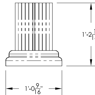
FRONT & SIDE VIEW SHORT PEDESTAL (VOGUEP114)
