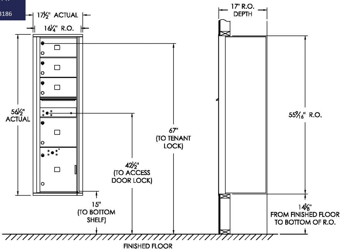
COMPARTMENT CHART
