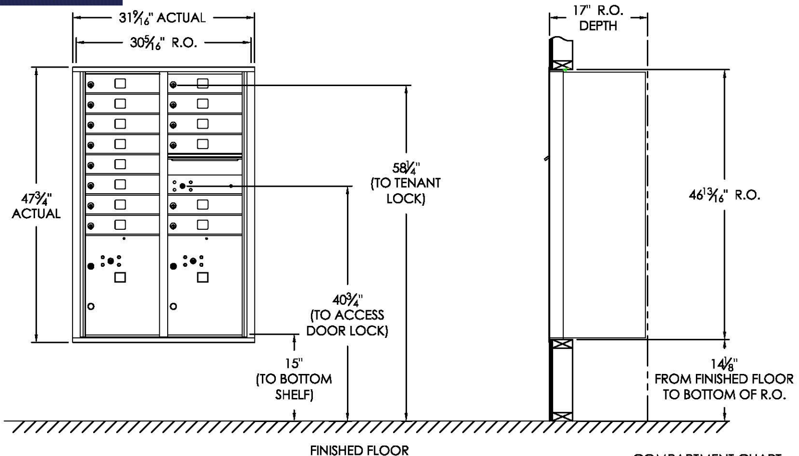
COMPARTMENT CHART
