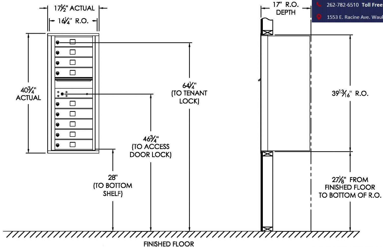
COMPARTMENT CHART
