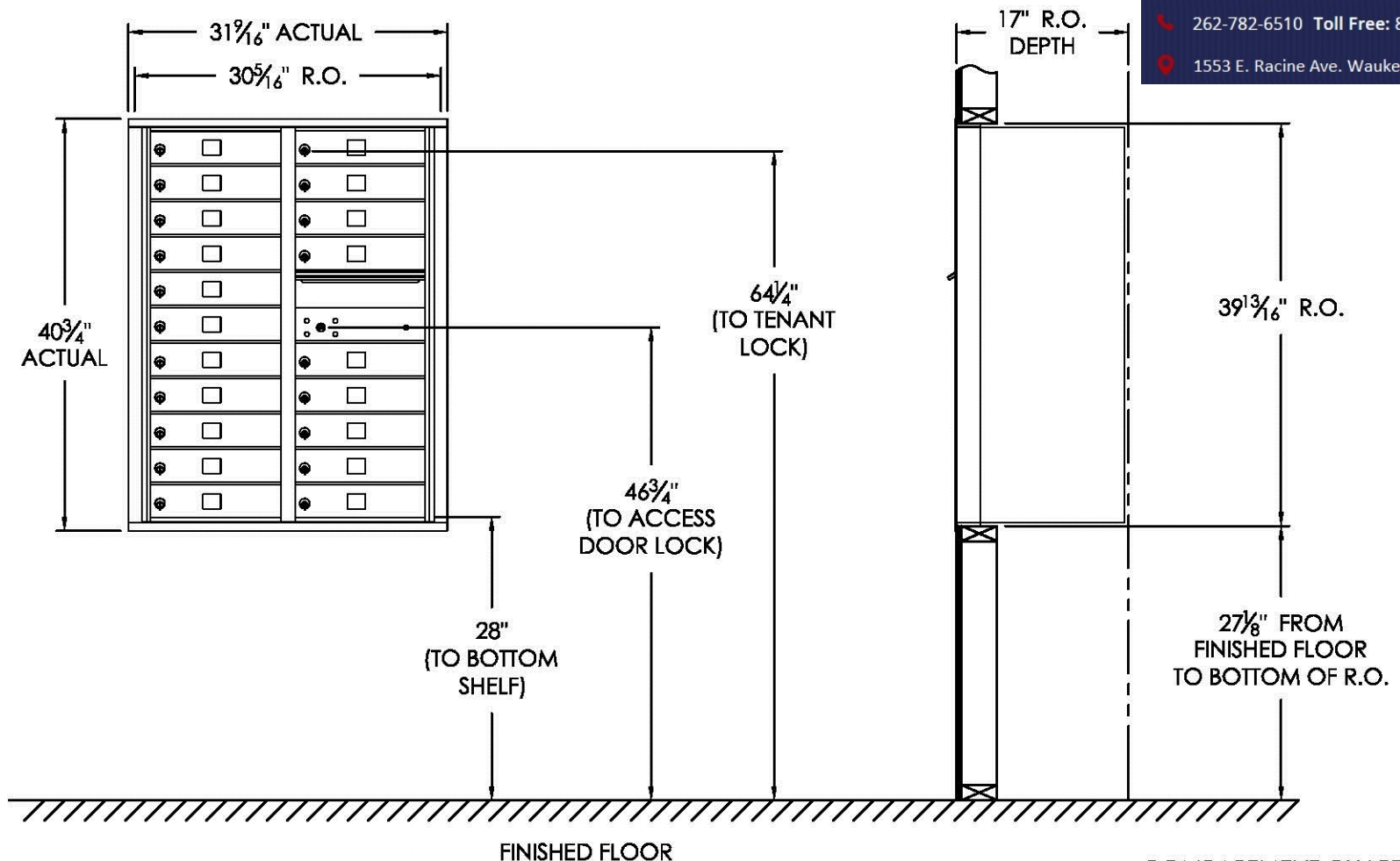
COMPARTMENT CHART
