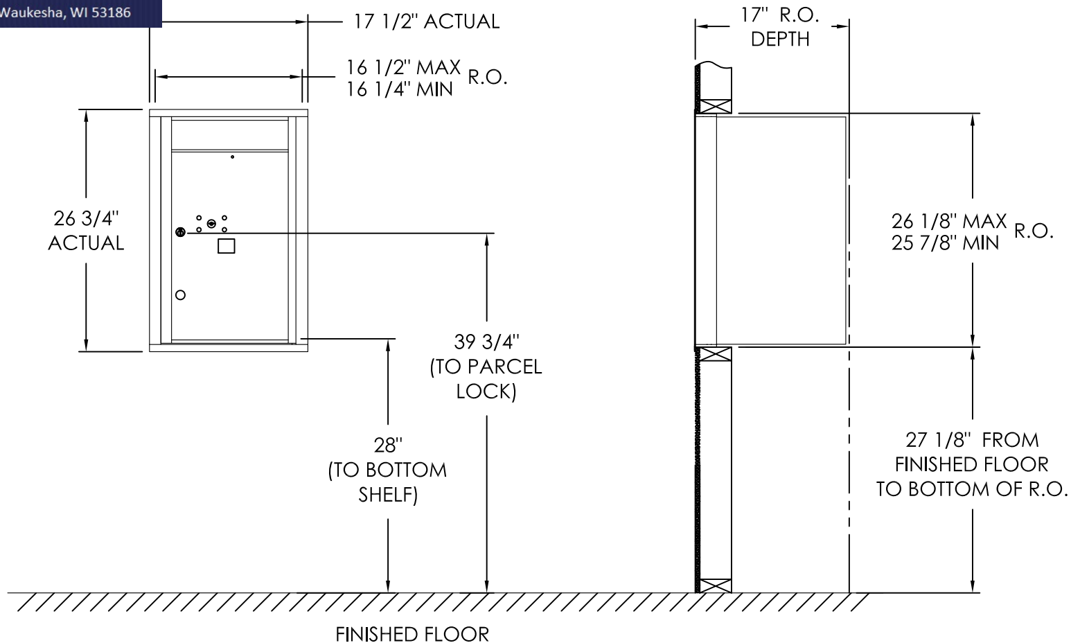
COMPARTMENT CHART
