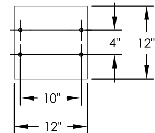
PEDESTAL BASE BOLT PATTERN
