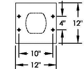
PEDESTAL DETAIL
