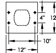
PEDESTAL DETAIL
