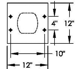
PEDESTAL DETAIL
