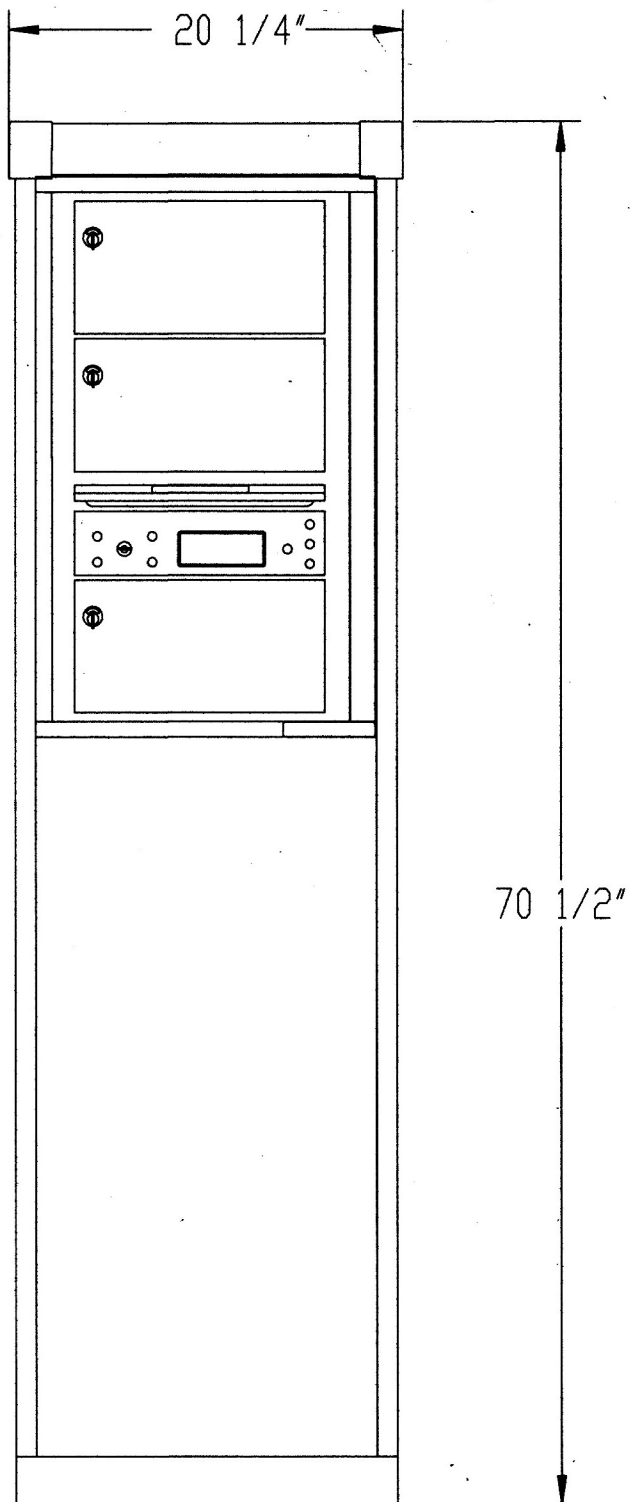
vario Depot medium with 4CET6-XL
