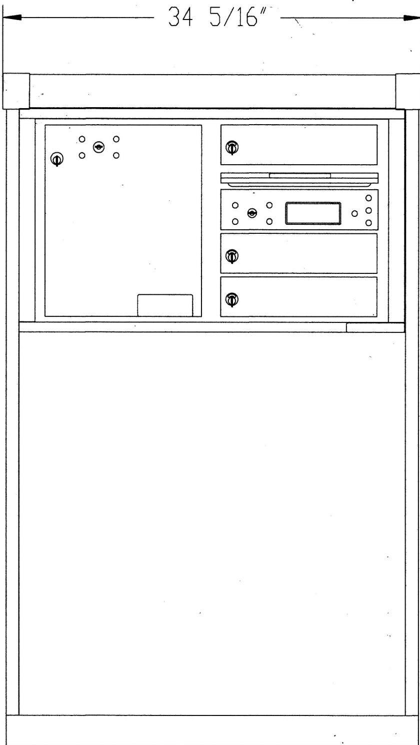
vario Depot small with 4CBT23
