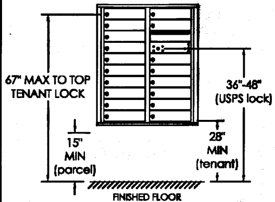
USPS INSTALLATION EXAMPLE
